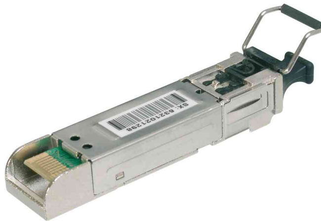
SFP Modul LWL-LC Duplex, Multimode
