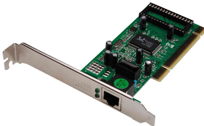
PCI Gigabit Ethernet RJ45 Netzwerkadapter
